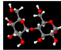
Maltose
