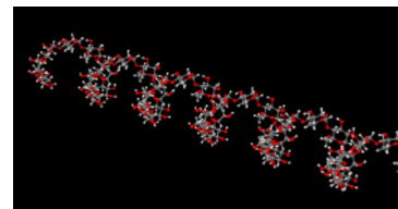
Amylose
