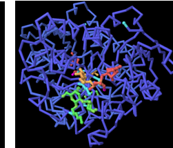
Glycosyltransferase
