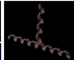
Amylopectin
