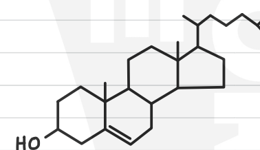
cholesterol
