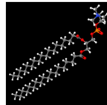
Phospholipid
