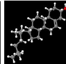
Cholesterol
