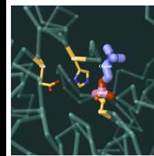
Acetylcholin-esterase
