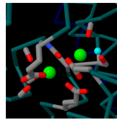
Sodium-Potassium Pump
