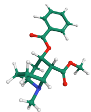
Cocaine
