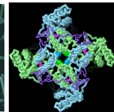
TRPV channel
